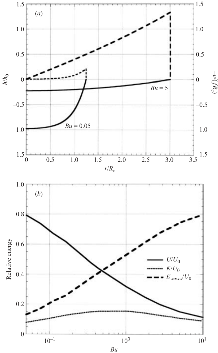
FIGURE 3. Final steady state according to the standard adjustment model §4. (a) Two adjusted velocity (dashed line) and height (solid line) profiles resulting from the same initial density anomaly ( h = h_0 , r = R_c ) are plotted for two different deformation radii Bu = 0.05 and Bu = 5 . (b) Relative potential U/U_0 , kinetic K/U_0 and wave energy E_{wave}/U_0 of the final adjusted state as a function of the Burgers number.
