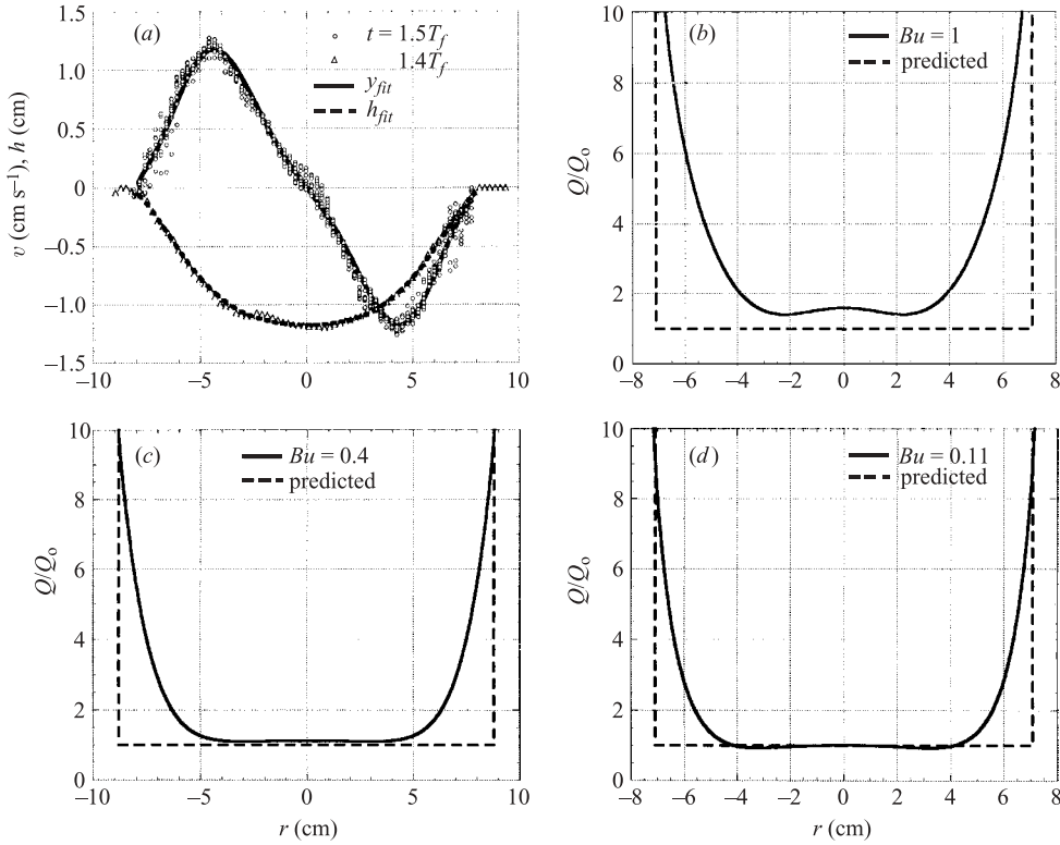
FIGURE 12. Potential vorticity profiles for (b) Bu = 1 , (c) 0.4 and (d) 0.11, deduced from independent measurements of velocity and height fields. These two profiles are fitted with high-order polynomials (a). ---, PV profiles predicted by standard adjustment (§4); —, profiles measured in the experiment.
